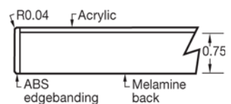
Profile Drawing
